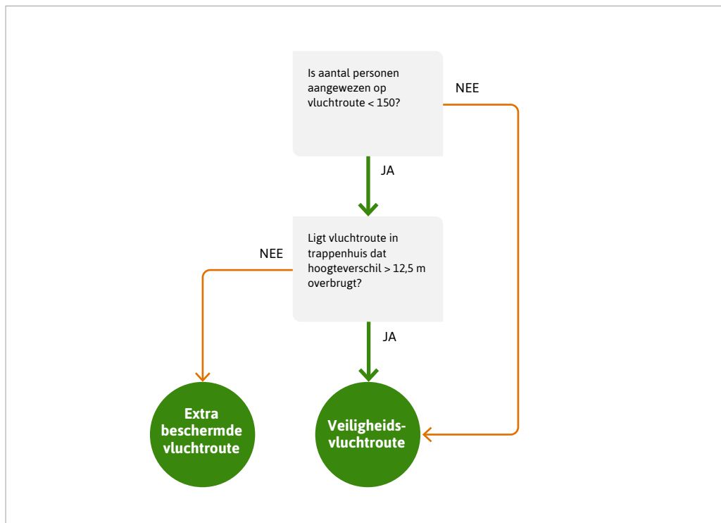
Stroomschema 3d.C
