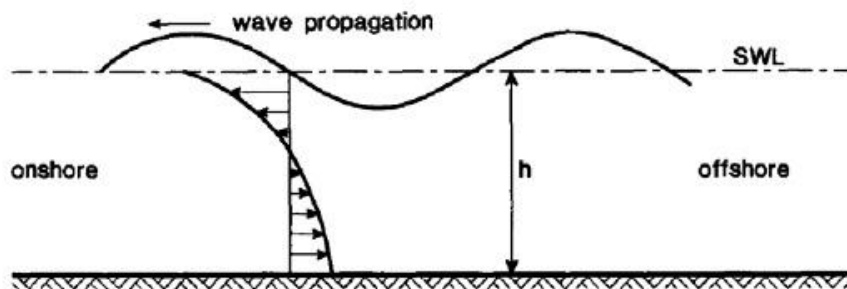
Figure 2.6 Schematized cross-shore velocity profile resulting from Stokes drift (Van Rijn, 1993).
