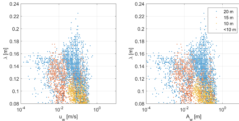
Figure 4.7. Ripple length versus orbital velocity (left) and ripple length versus orbital excursion (right).
