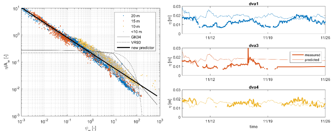
Figure 4.12. Left: Nondimensional ripple height versus wave mobility number. Lines denote the Grasmeijer & Kleinhans (2004) and Van Rijn (1993) model curves. The thick black line is the proposed new model. Right: measured and predicted ripple heights by the proposed model through time.
