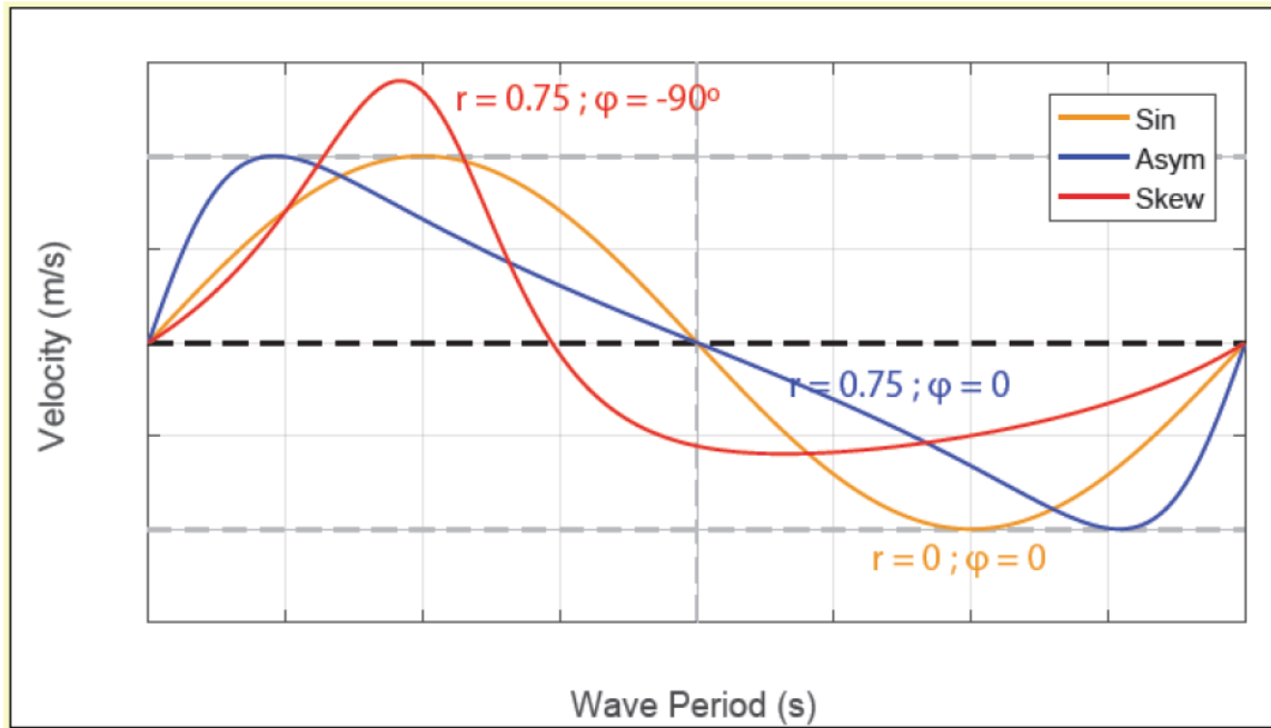
Figure 2.4 Shape of a perfectly sinusoidal, a skewed, and an asymmetric wave (from: Treurniet, 2018). The definition of the non-linearity parameter ( r ) and phase ( \phi ) are given by Abreu et al. (2010).
