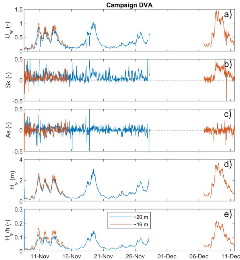
Figure 3.1 Time series of (a) the wave orbital velocity amplitude, (b) skewness, (c) asymmetry, the significant wave height (d), and the relative wave height (e) during the Ameland lower shoreface campaign in November 2017.
