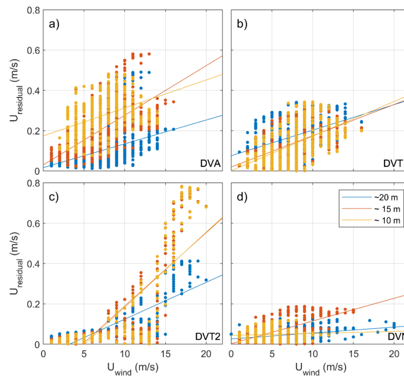
Figure 3.15 Scatterplots of the regional (nearby KNMI station) wind speed and residual current magnitude for different depths (colours) and locations (subplots a-d) of the Dutch lower shoreface. Lines represent linear least squares regressions on the data.
