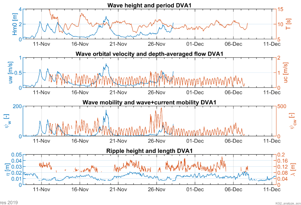
Figure B.5 Timeseries of surface wave characteristics, (wave orbital) velocity, wave and current mobility parameters, and the accompanying bedform dimensions, for DVA-F1.
