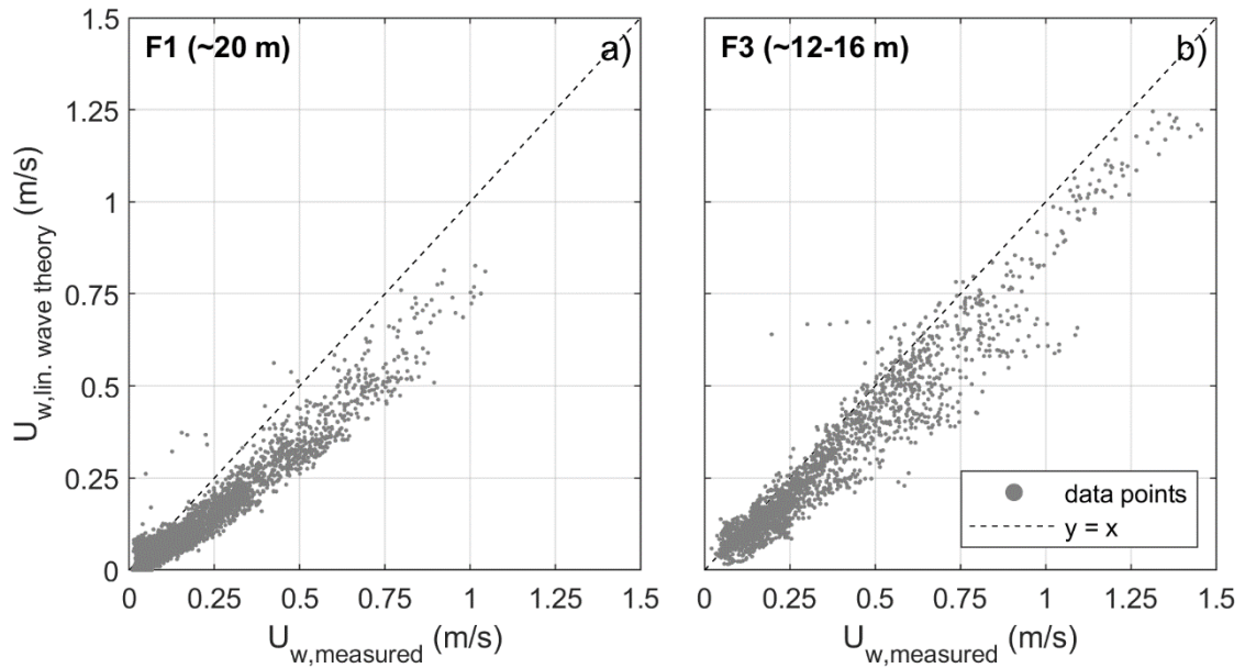
Figure 3.6 Scatterplots of the significant orbital velocity amplitude ( U_w ) determined by linear wave theory vs. the amplitudes derived from the ADV instruments, for ~20 m (a) and ~12-16 m (b) water depth.
