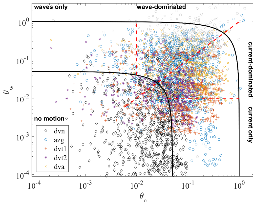
Figure 4.1. Measured wave- versus current-related Shields stress for all campaigns. Black lines indicate sheetflow and incipient motion. Red dashed lines show the boundaries between regions of wave or current dominance, according to Kleinhans (2005). Grey data points indicate moment with no SONAR data.
