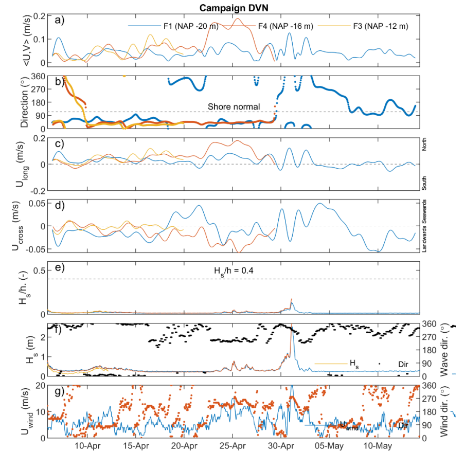
Figure 3.13 Campaign DVN: residual flow magnitude (a) and direction (b) at all frames; residual flow in longshore (c) and cross-shore (d) direction (see direction at right side of panels); breaker criterion at all frames (e); wave height (from observations) and direction (from the wave transformation matrix at the most offshore frame) (f); and measured wind velocity and direction at KNMI station IJmuiden (g).
