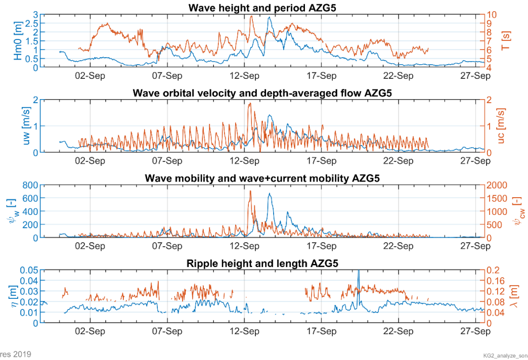
Figure B.4 Timeseries of surface wave characteristics, (wave orbital) velocity, wave and current mobility parameters, and the accompanying bedform dimensions, for AZG-F5.
